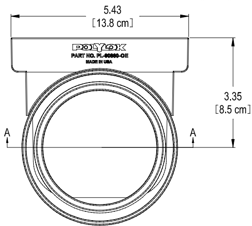
POLYLOK TRENCH DRAIN OUTLET END CAP PART NO'S. PL-90860-OE (BLACK) PL-90860-OEG (GREY) MATERIAL - ABS COLOR - BLACK AND GREY
